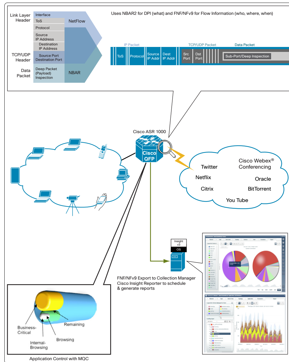
Figure 1. Cisco AVC Solution
