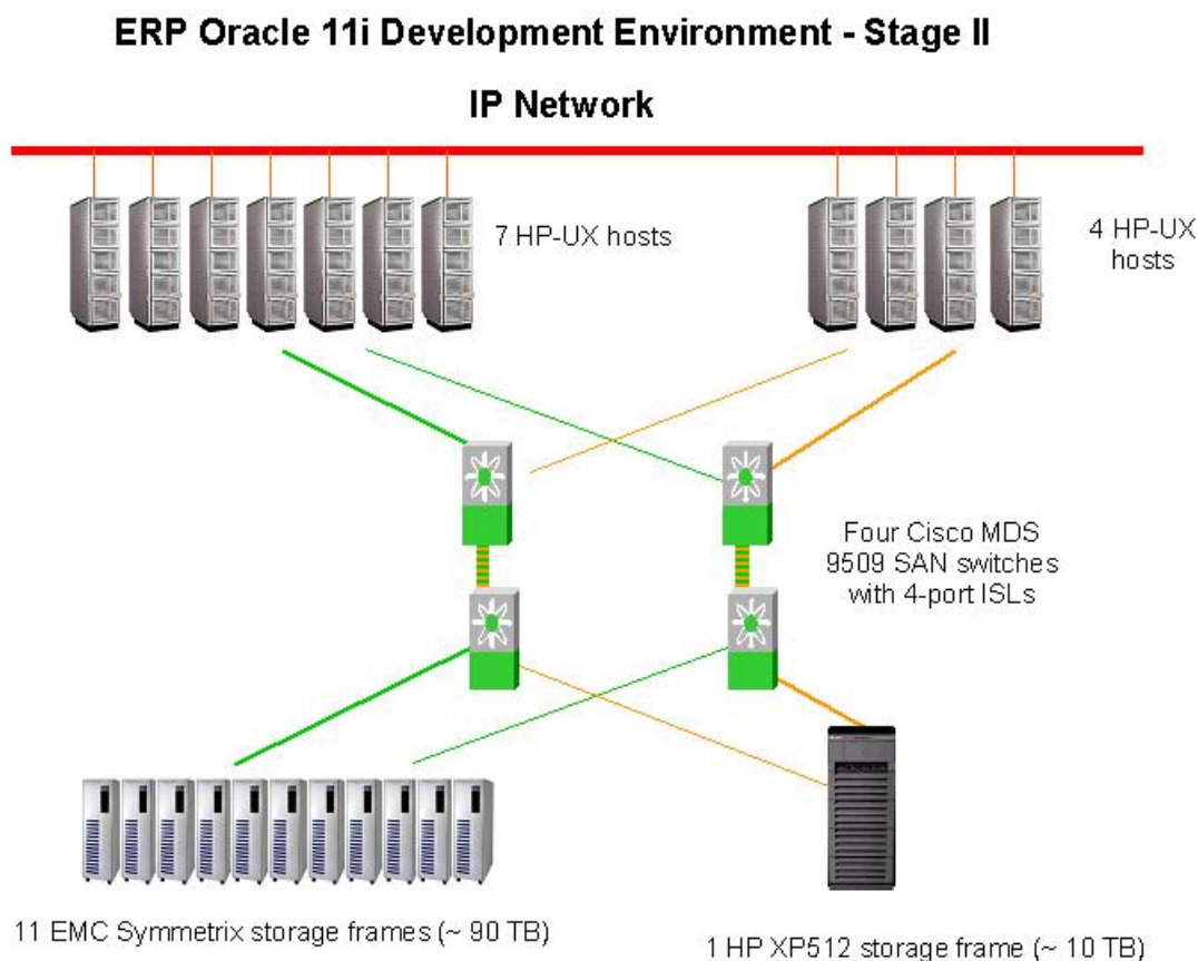
Figure 12. Consolidated ERP Oracle 11i Development SAN (After Stage II)
