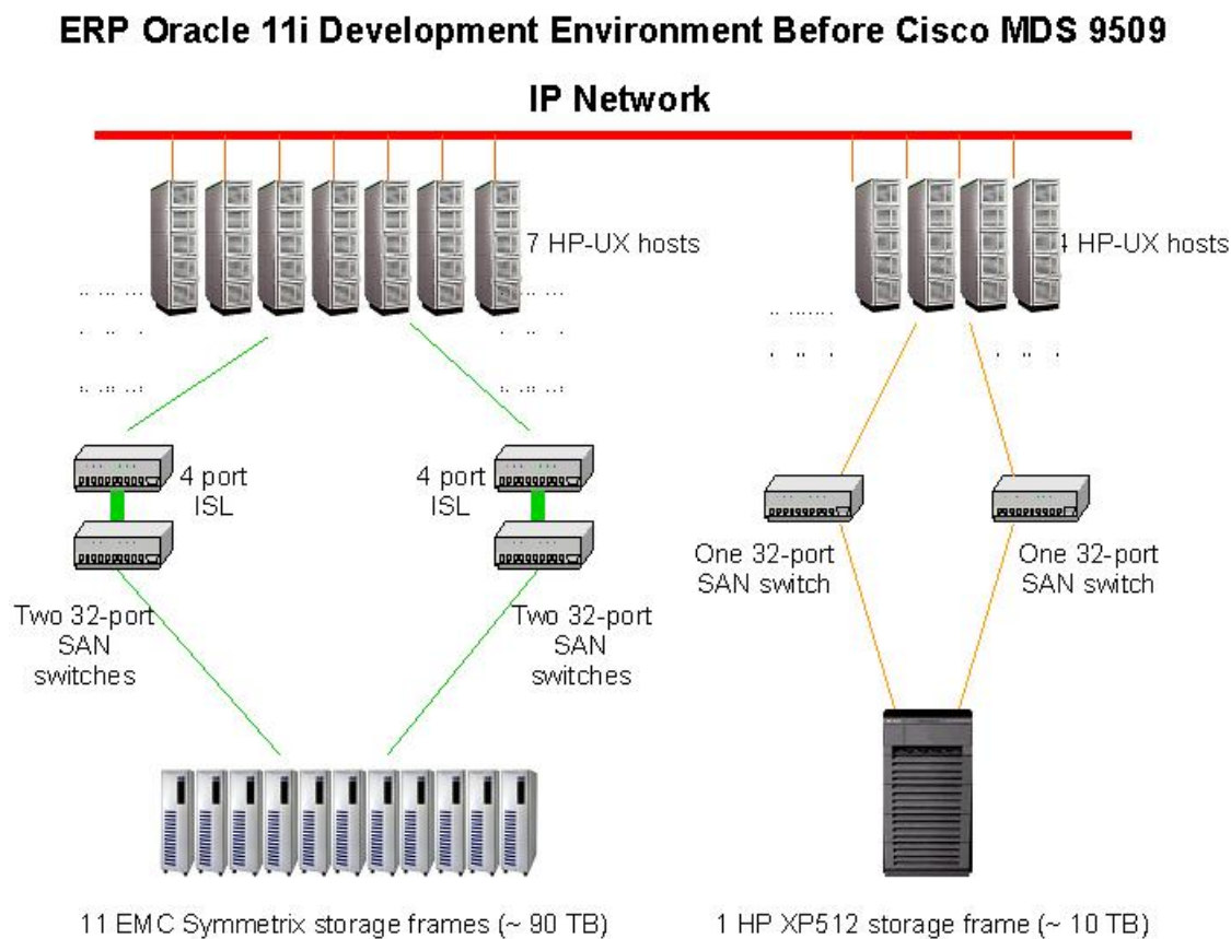
Figure 10. ERP Oracle 11i SAN Islands Prior to Implementation of Cisco MDS 9509 and Cisco MDS 9513 Switches
