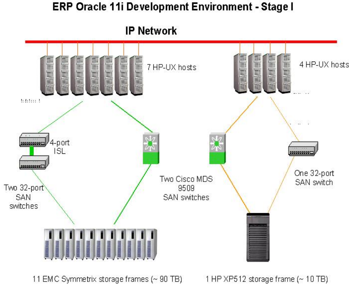
Figure 11. ERP Oracle 11i Development SAN Islands after Migration Stage 1
