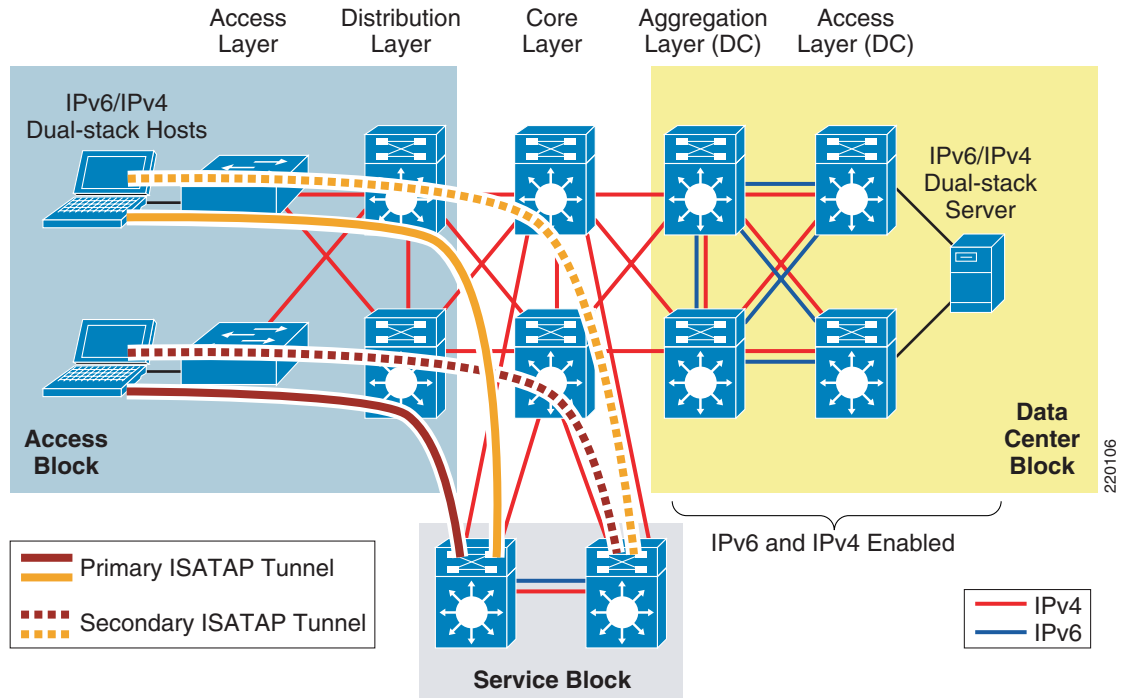
Figure 6 Service Block Model—Connecting the Hosts (ISATAP Layout)
