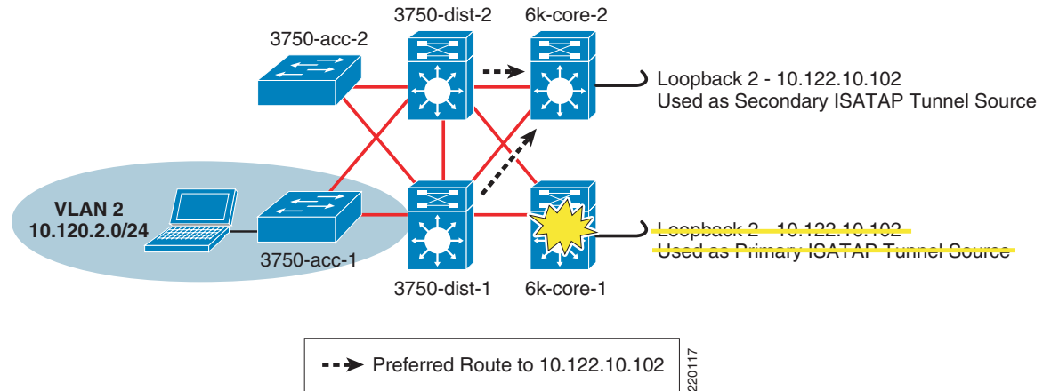
Figure 17 HME1—Preferred Route for 6k-core-2 After Failure of 6k-core-1
