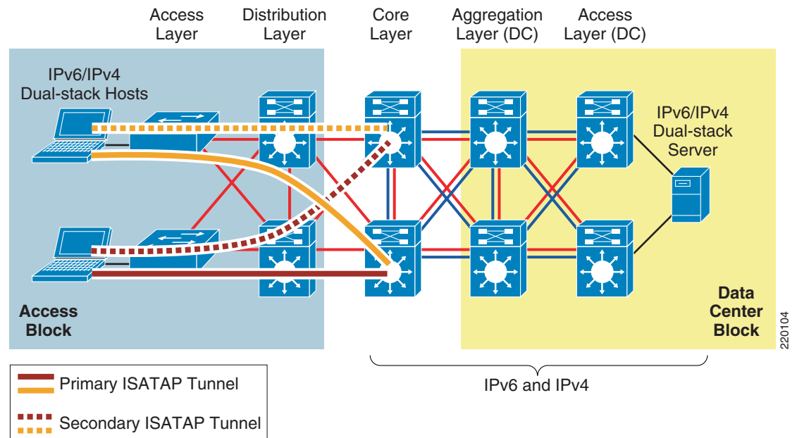
Figure 4 Hybrid Model Example 1
