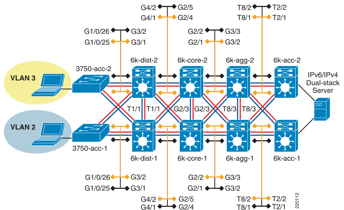
Figure 12 DSM Network Topology—Physical Ports
