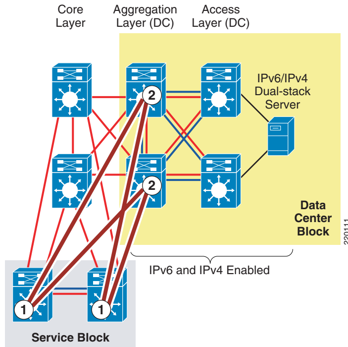
Figure 10 QoS Policy Implementation—SBM (ISATAP and Manually-Configured Tunnels)
