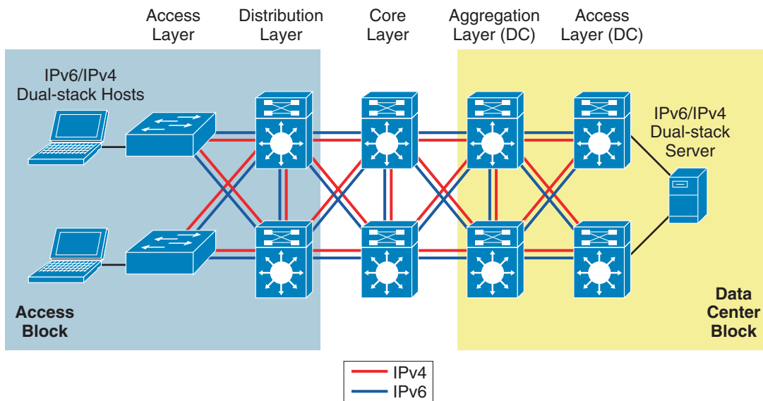
Figure 1 Dual-Stack Model Example
