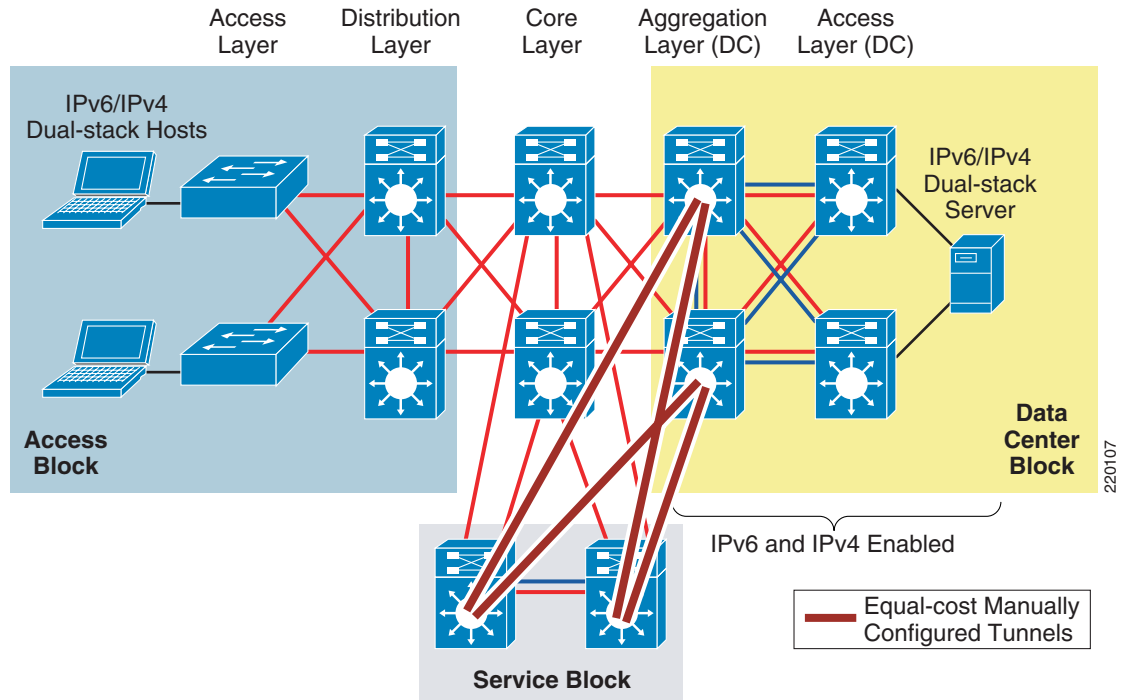
Figure 7 Service Block Model—Connecting the Data Center (Manually-Configured Tunnel Layout)
