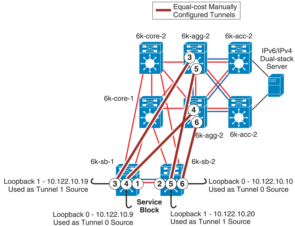
Figure 19 SBM Manually-Configured Tunnel Topology
