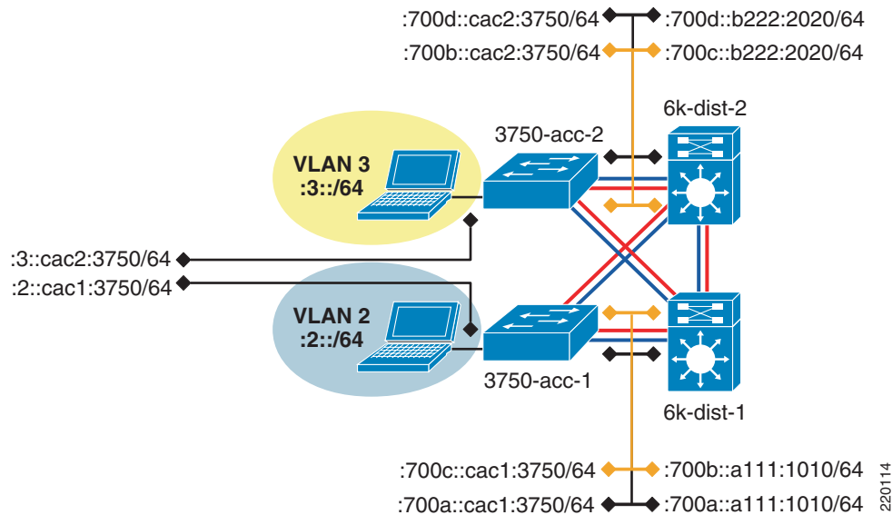
Figure 14 DSM Topology—Routed Access Design
