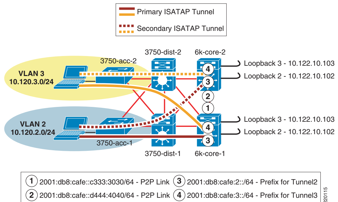
Figure 15 HME1 Network Topology
