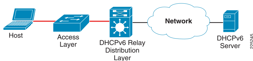
Figure 11 DHCPv6 Relay Placement in the Campus
