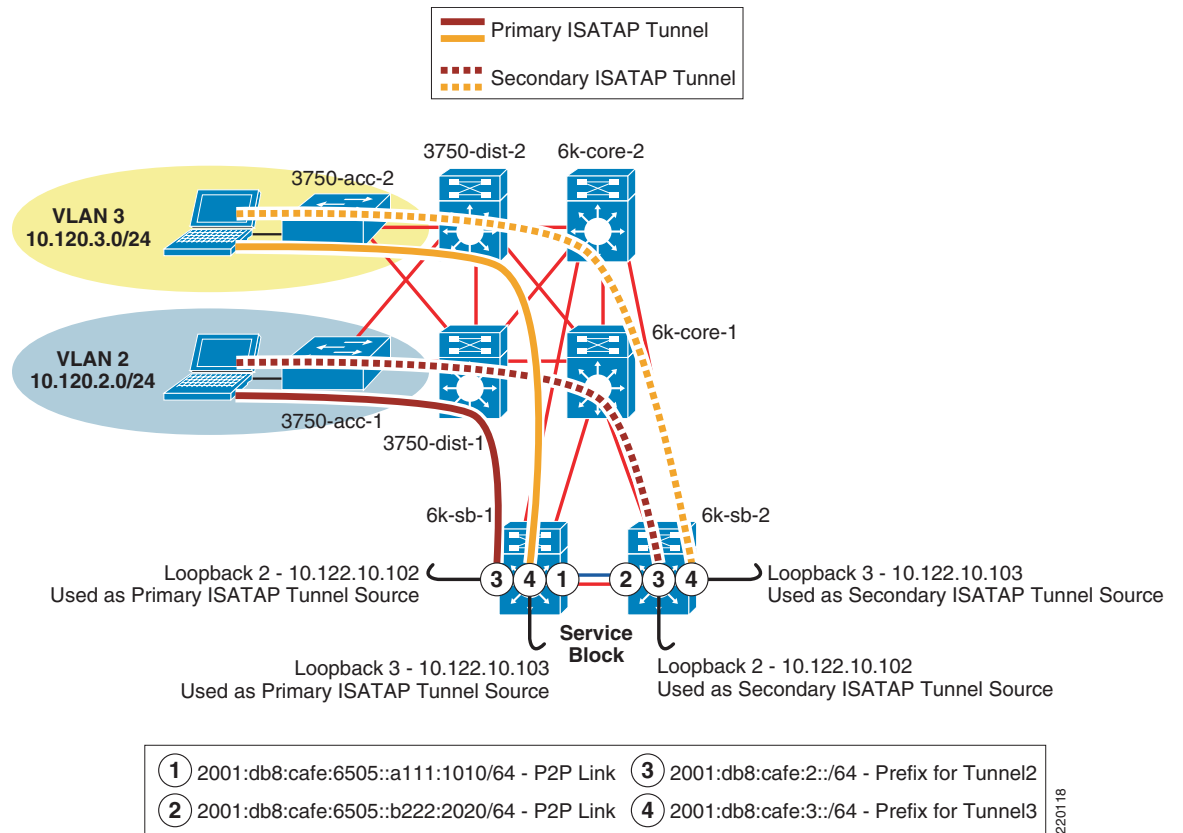
Figure 18 SBM ISATAP Network Topology
