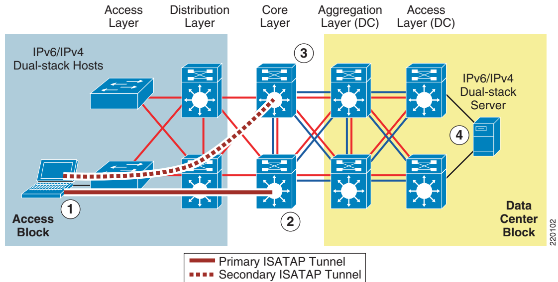
Figure 2 Hybrid Model Example 1—Connectivity Flow
