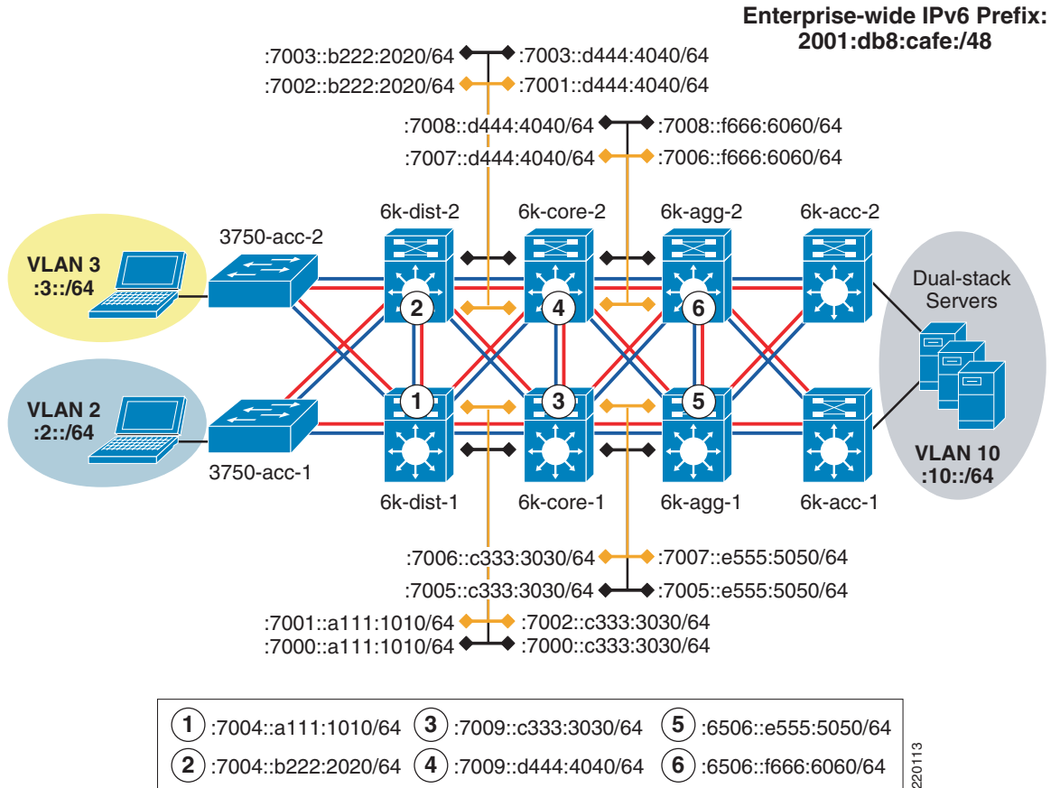
Figure 13 DSM Network Topology—IPv6 Addressing
