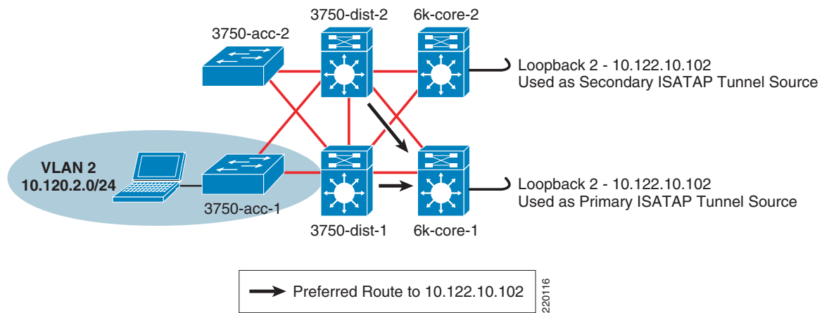
Figure 16 HME1—Preferred Route for 6k-core-1
