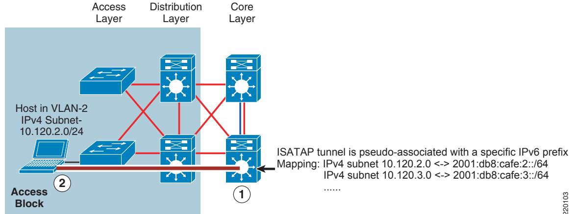
Figure 3 Hybrid Model Example 1—ISATAP Tunnel Mapping
