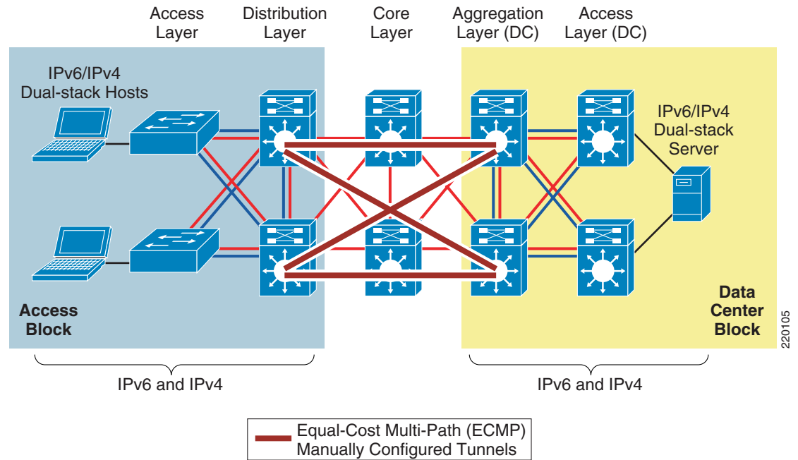
Figure 5 Hybrid Model Example 2
