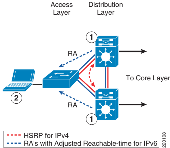
Figure 8 Host Receiving an Adjusted NUD Value from Distribution Layer
