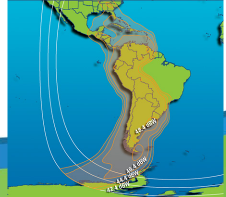
Ku-Band Americas Beam Peak up to 49.4 dBW
